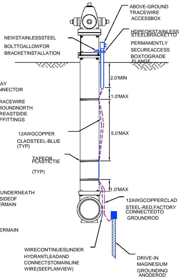
HYDRANT-SECTION VIEW
