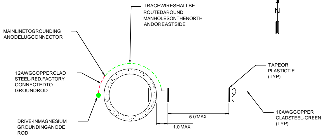
SEWER MANHOLE-PLAN VIEW
